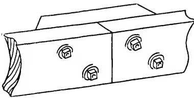
FISHED JOINT-A
